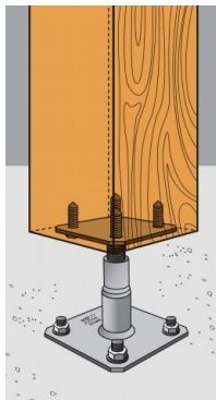
Fixation pied poteau APB100/150 sur support rigide
